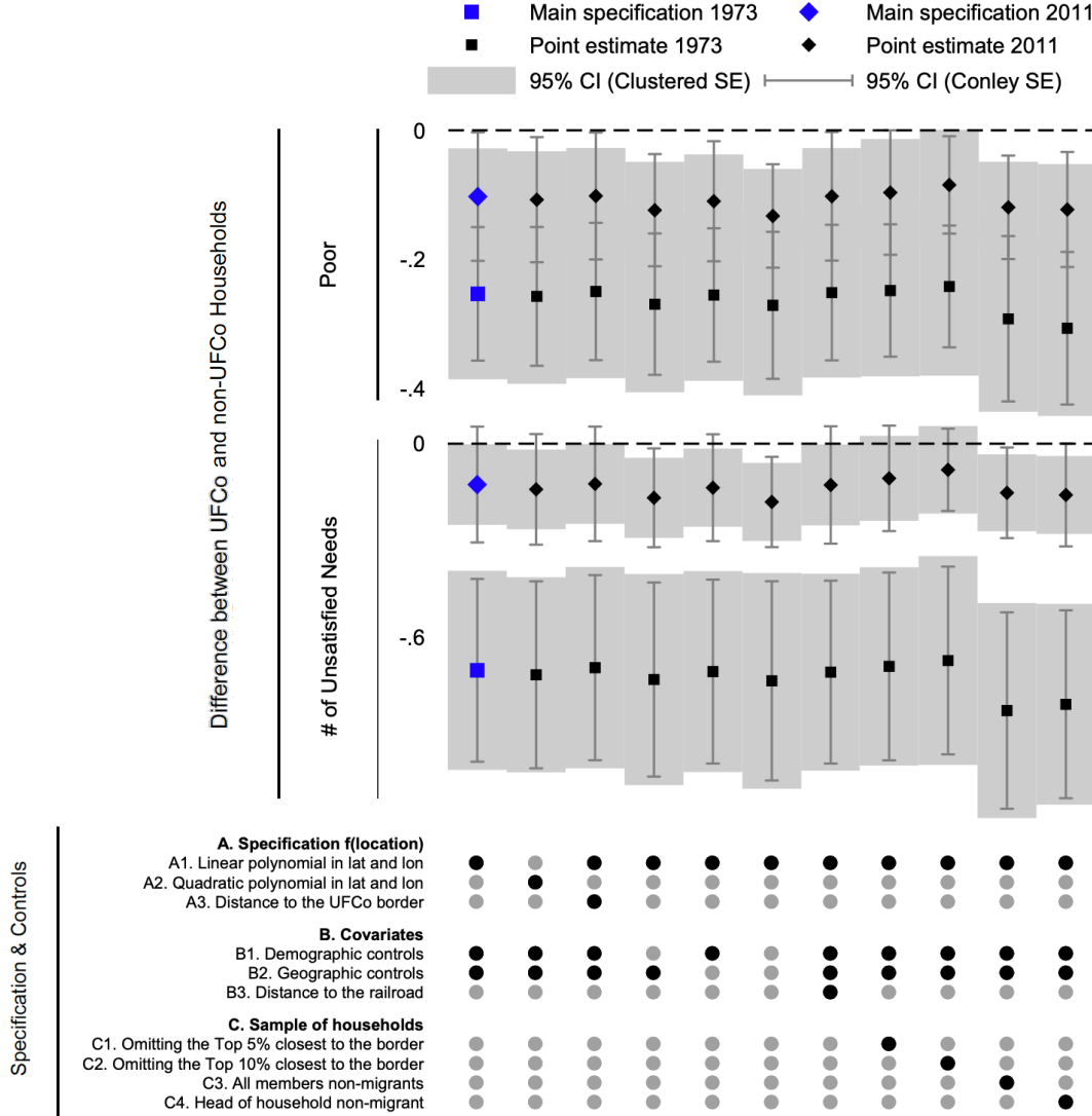
Figure 14: Robustness checks, Main Specification, Dynamic UFCo Effect (Part 1/2)
