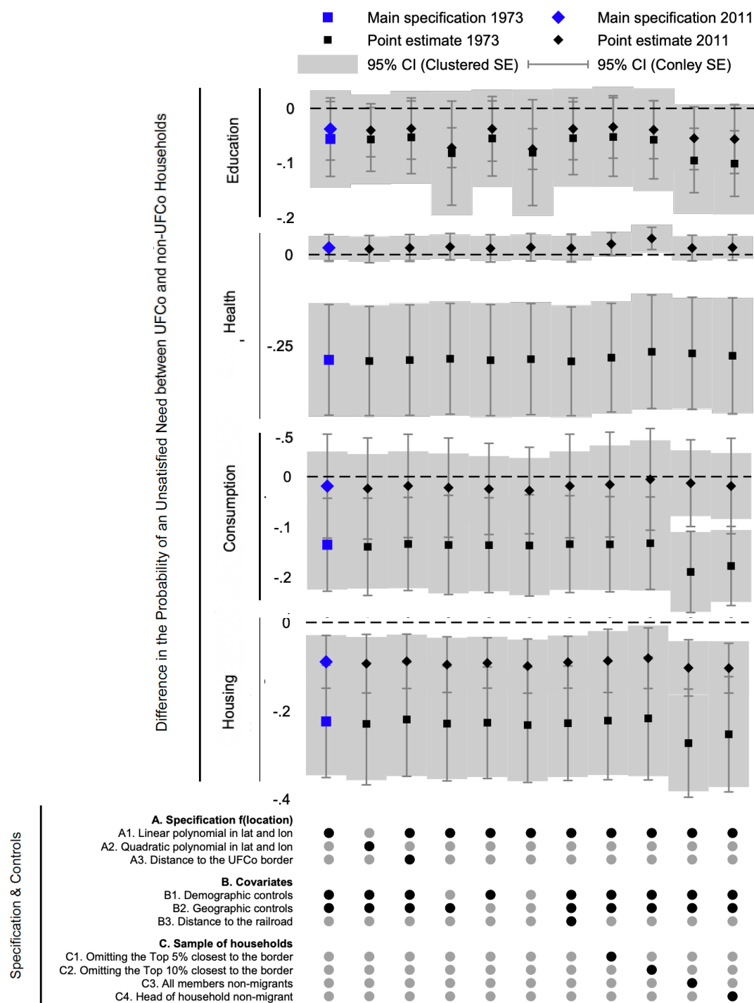
Figure 15: Robustness checks, Main Specification, Dynamic UFCo Effect (Part 2/2)
